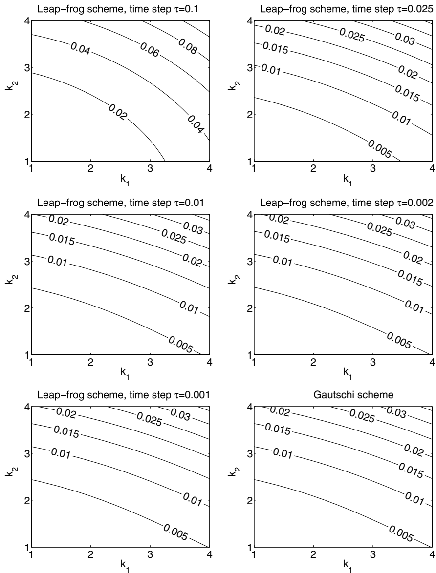
Fig. 7. Absolute value of the angular frequency errors for the leap frog scheme with different time steps and for the Gautschi scheme, mesh size h = 1/20 , deformation angle \theta = \pi/4 .
