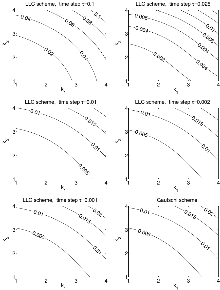
Fig. 9. Absolute value of the angular frequency errors for the LLC scheme with different time steps and for the Gautschi scheme, mesh size h = 1/20 , deformation angle \theta = \pi/3 .
