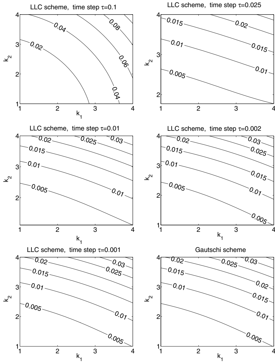
Fig. 10. Absolute value of the angular frequency errors for the LLC scheme with different time steps and for the Gautschi scheme, mesh size h = 1/20 , deformation angle \theta = \pi/4 .
