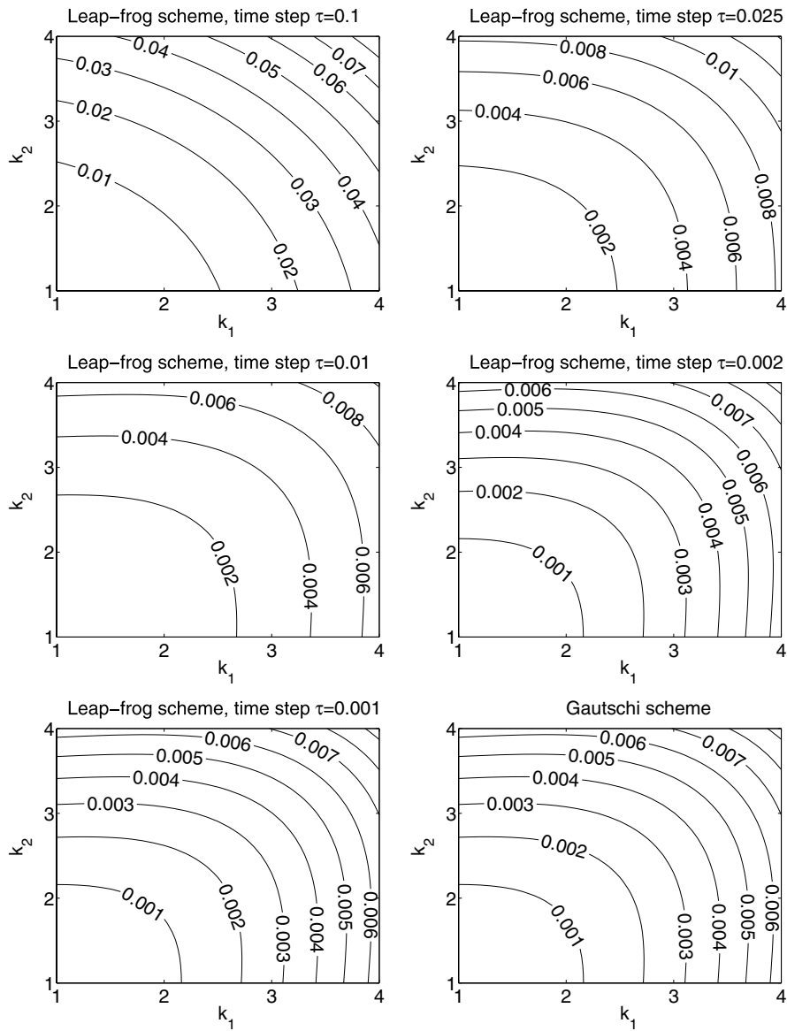
Fig. 5. Absolute value of the angular frequency errors for the leap frog scheme with different time steps and for the Gautschi scheme, mesh size h = 1/20 , deformation angle \theta = \pi/2 .
