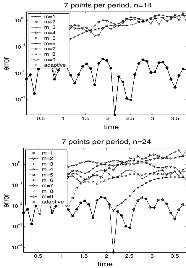
Fig. 11. Error evolution of the Gautschi scheme for 14 \times 14 \times 14 (top) and 24 \times 24 \times 24 (bottom) meshes for different Krylov subspace dimensions m . The step size corresponds to 7 points per time period.
