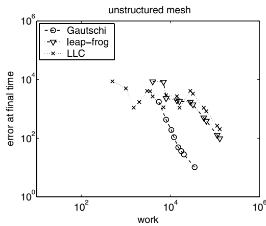
Fig. 17. Unstructured mesh. Errors at the final time against the corresponding computational work for homogeneously distributed frequencies in the source term. The work is measured in the Q units (see Section 6.4).
