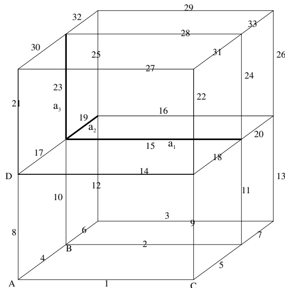
Fig. 3. Three nonparallel edges a_1, a_2, a_3 and the degrees of freedom (with a local numbering) that appear in Eq. (5.7) for edge a_1 .
